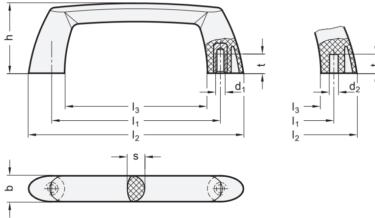
elesa Original design M.943
