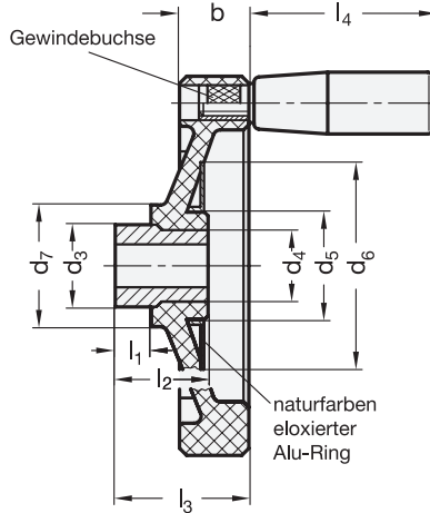
elesa Original design VDN.FP-A
